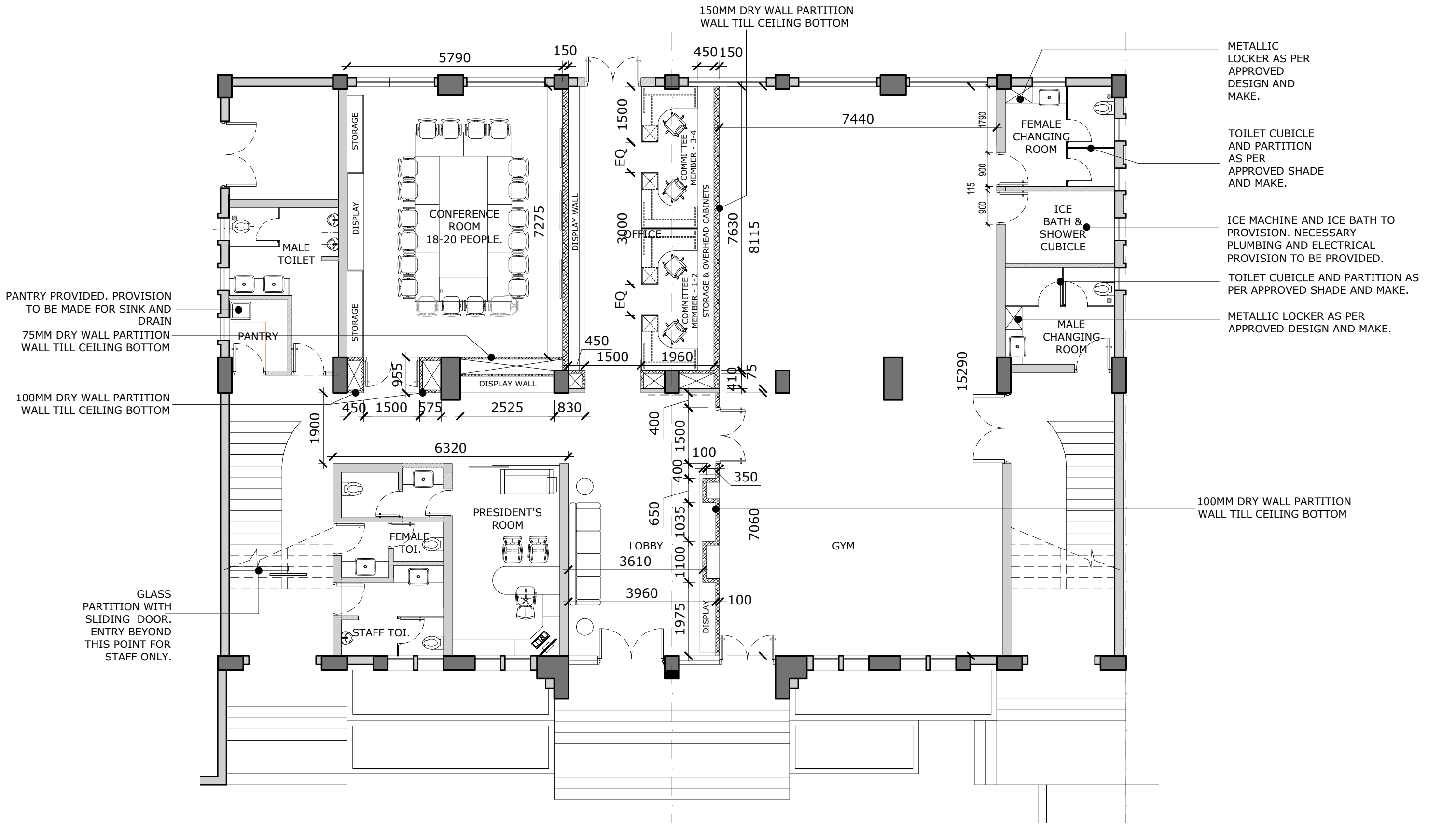
PLAN SCALE 1:100
